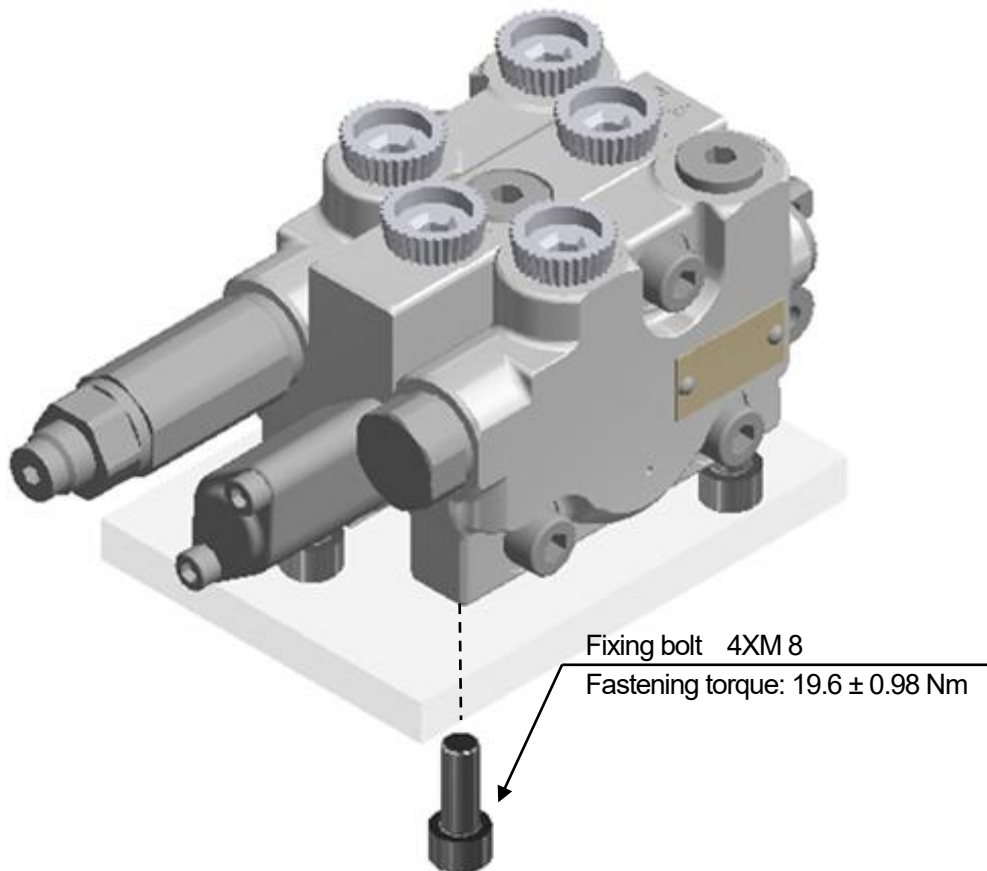
Fig. 7-1 Installation into Machine
