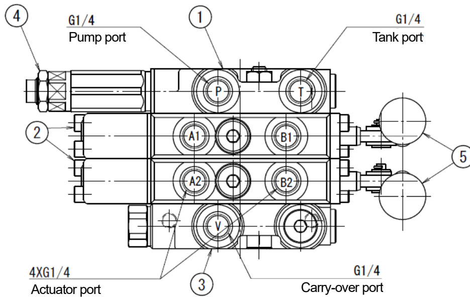
Fig. 2-3 Example of V-port Type
