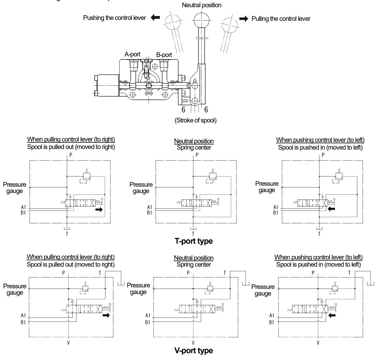
Fig. 3-2 About Ports
