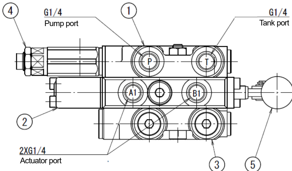
Fig. 2-2 Example of T-port Type
