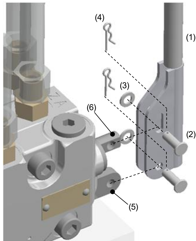
Fig. 7-3 How to Mount the Set of Control Lever Parts
