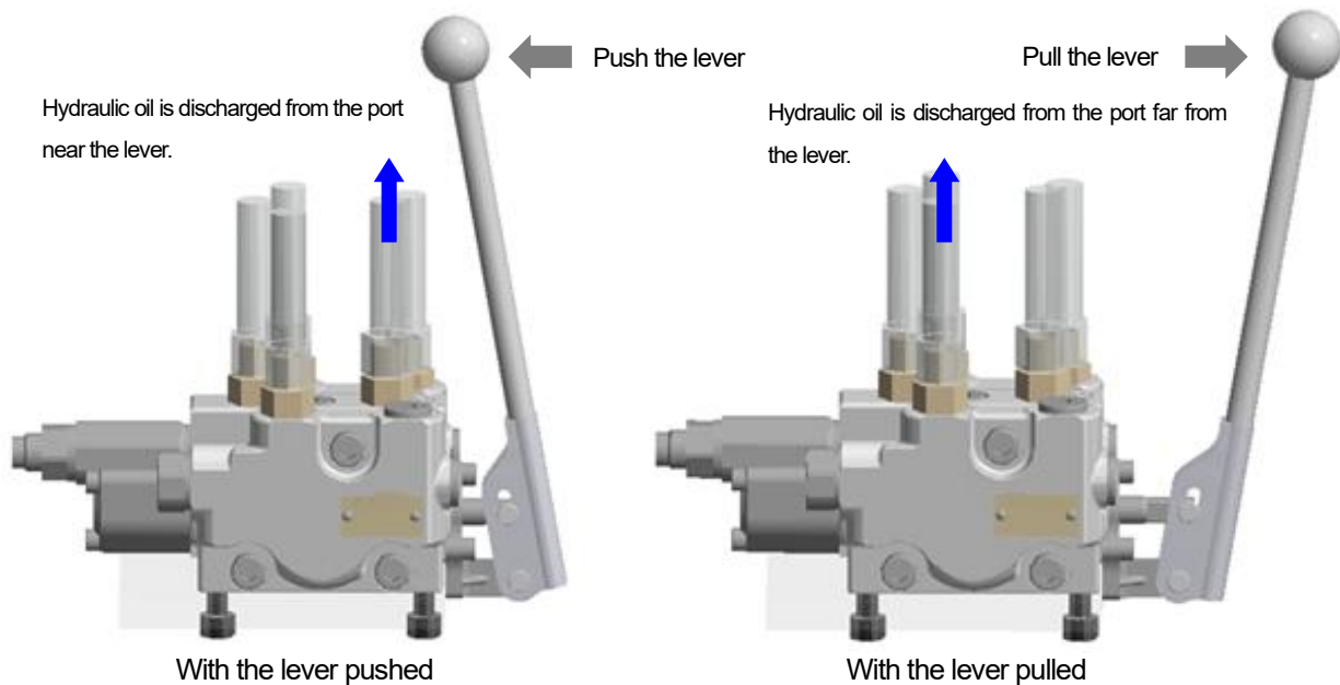
Fig. 8-1 Discharge Port of Hydraulic Fluid
