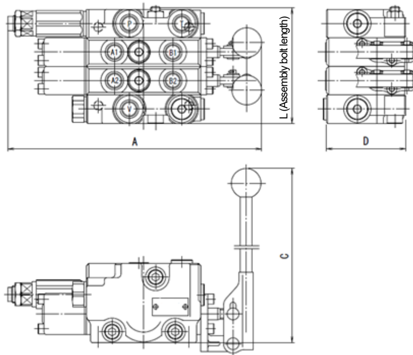
Fig. 3-1 Outline Drawings
