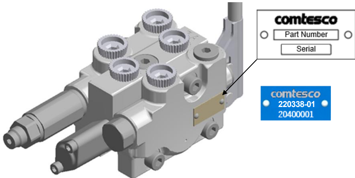
Fig. 4-4 Nameplate
